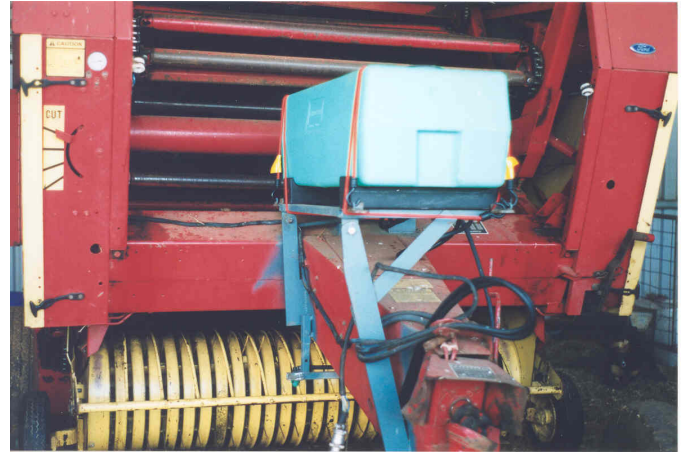
Figure 1. Spray applicator on baler
